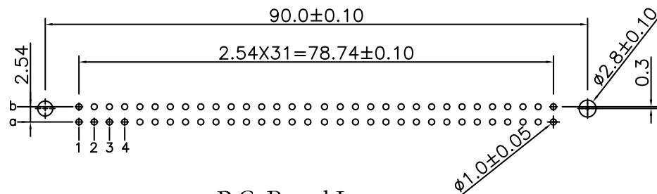
P.C. Board Layout (Tolerance:±0.05)
